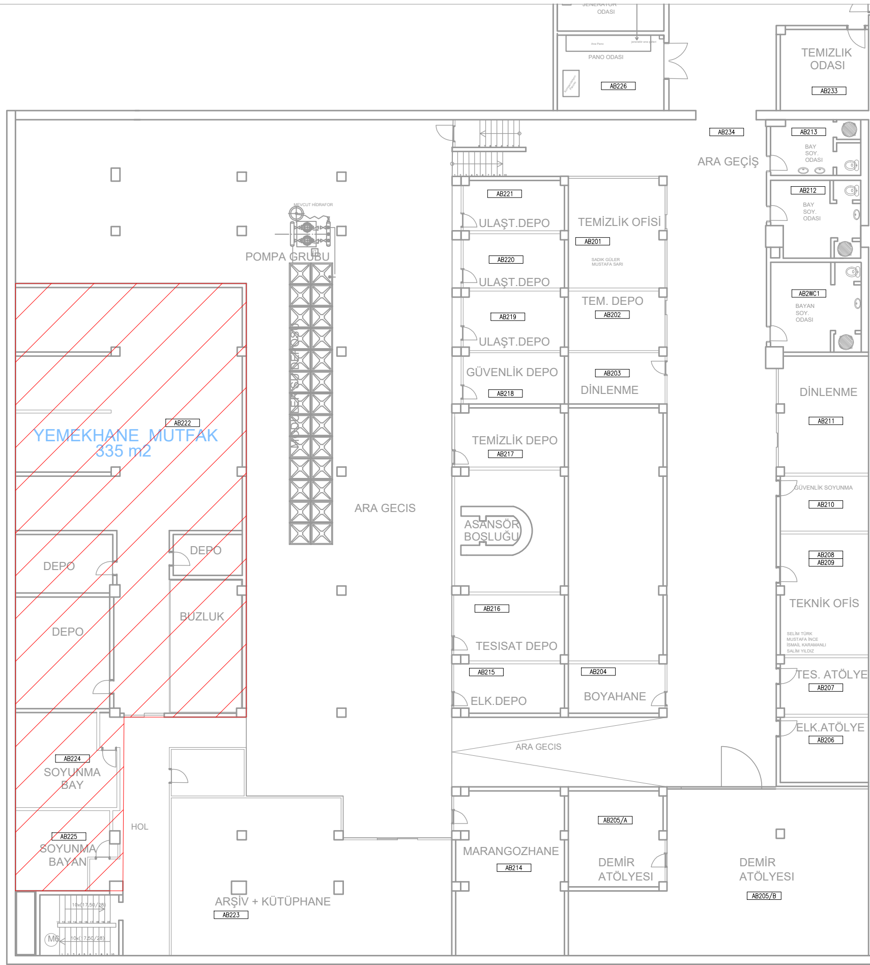
A BLOK 2.BODRUM KAT PLANI
